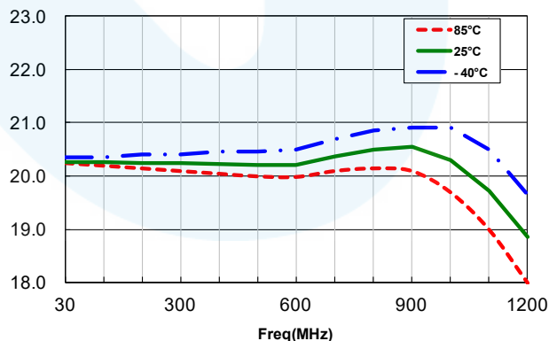
Frequency vs. Gain
