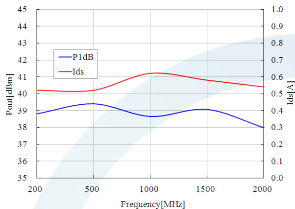
Ids vs. Frequency (@P1dB)
