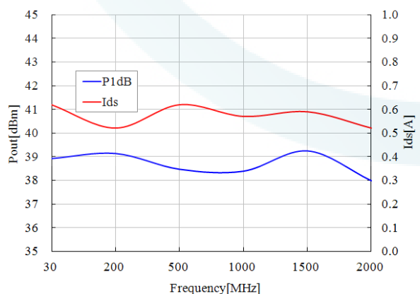
P1dB &amp; Ids vs. Frequency (under 200MHz)
