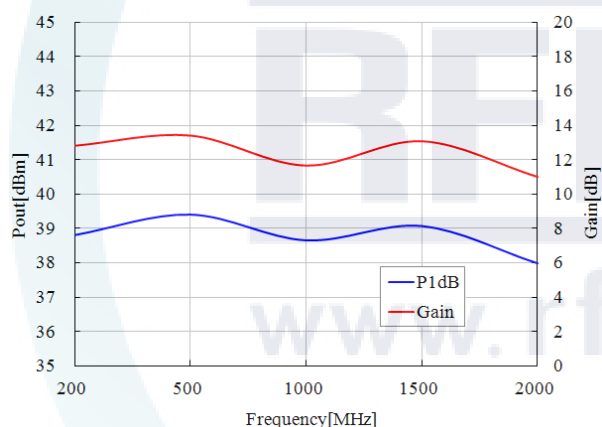
Power Gain vs. Frequency (@P1dB)
