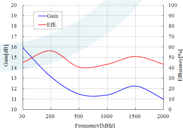
Gain &amp; Efficiency vs. Frequency @P1dB (under 200MHz)
