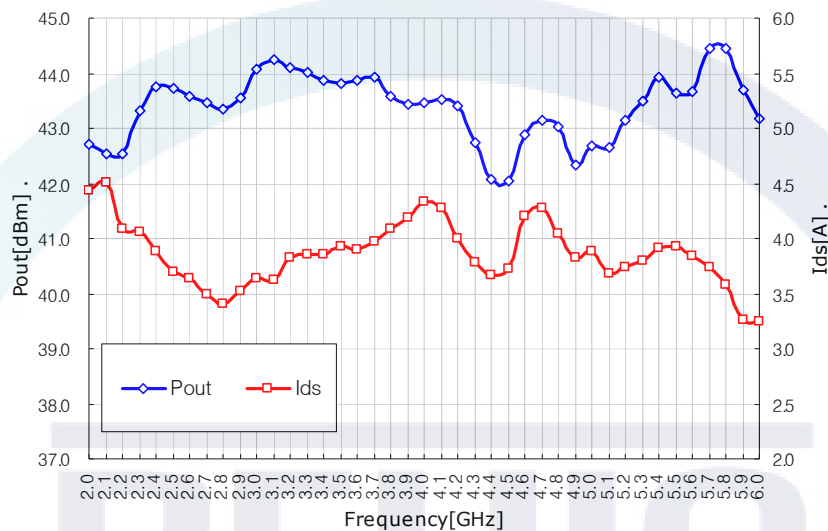
Output Power @ P_{in}=6\text{dBm} & I_{ds} vs. Frequency
