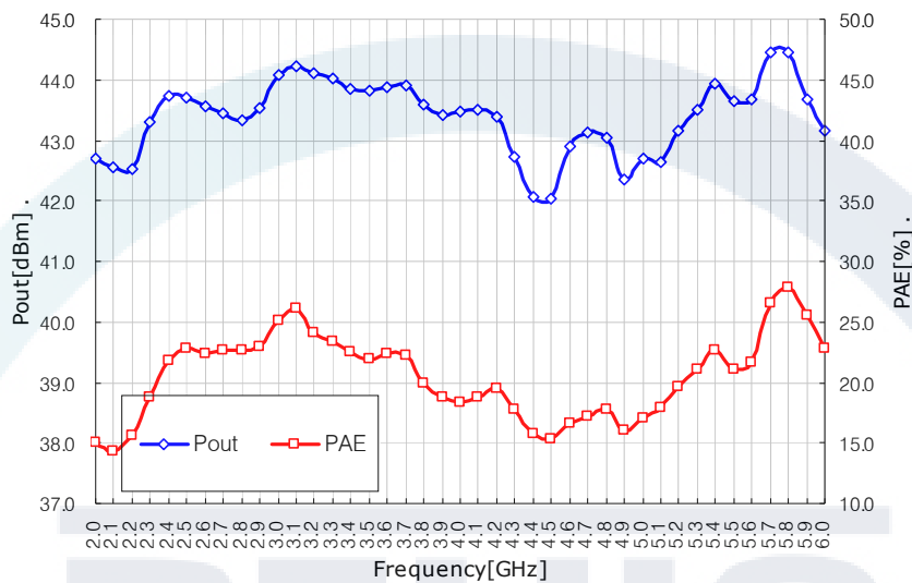
Output Power @ Pin=6dBm &amp; PAE vs. Frequency
