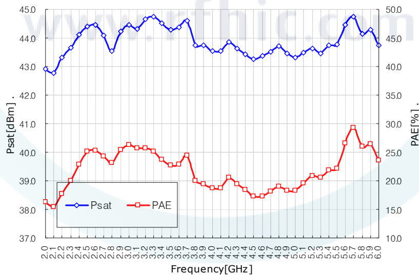
Saturation Power &amp; PAE vs. Frequency
