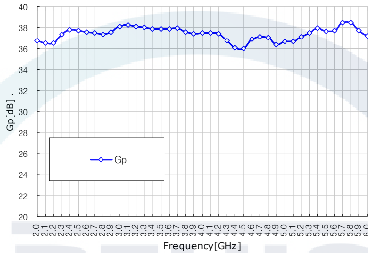
Power Gain @ P_{in}=6\text{dBm} vs. Frequency
