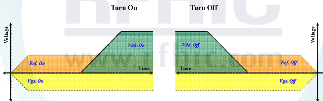
- Sequence Timing Diagram -
