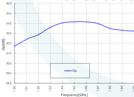
Power Gain @ Pin=14dBm vs. Frequency
