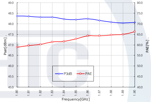
P3dB & PAE vs. Frequency
