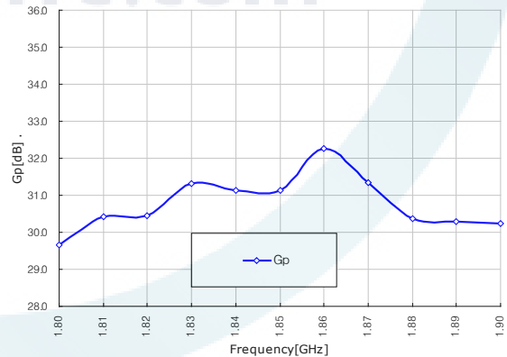
Power Gain @ P3dB vs. Frequency
