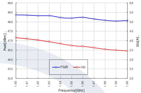
P3dB & Ids vs. Frequency
