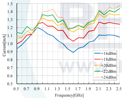
Ids @ Pin vs. Frequency
